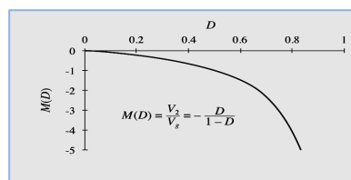
O/P Voltage gain vs %D
