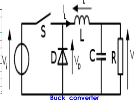
Buck converter
