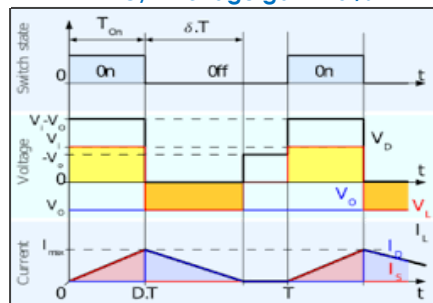
DCM mode
